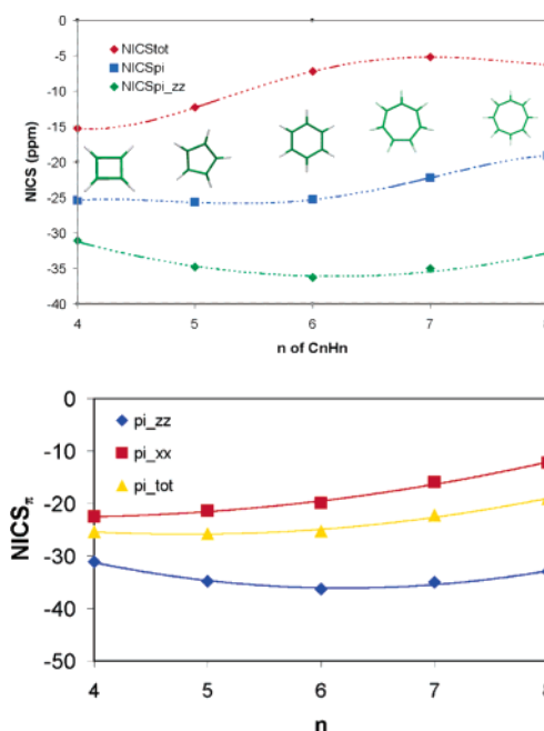
Figure 9. (a) Isotropic NICS, NICS_{\pi} , and NICS_{\pi zz} component, and (b) NICS_{\pi} tensor components against the ring size n in a series of six \pi electron annulenes at the ring centers (in ppm).
