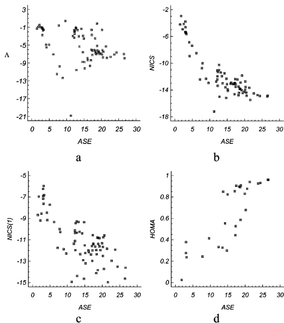
Figure 22. Dependence of \Delta , NICS, NICS(1), and HOMA vs ASE for all aza and phospha derivatives of furan, thiophene, pyrrole, and phosphole (including parent systems): (a) exaltation of magnetic susceptibility vs ASE (correlation coefficient = -0.3447 ; 72 data); (b) NICS vs ASE (correlation coefficient = -0.8588 ; 72 data); (c) NICS computed 1 Å above the ring centers vs ASE (correlation coefficient = -0.7456 ; 72 data); (d) HOMA vs ASE (correlation coefficient = 0.8360 ; 28 data).
